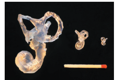
To better understand anatomy structure, inner ear fossils are scanned and printed to reveal details otherwise invisible to the human eye (middle and right: original size)
